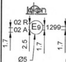
Prüfnummer / layout of approval marking
